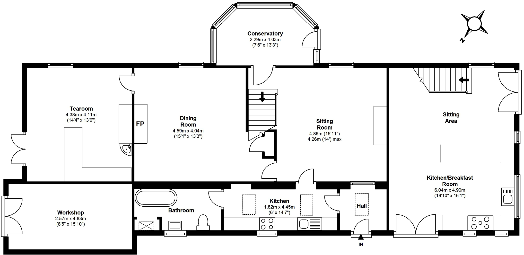
Ground Floor
